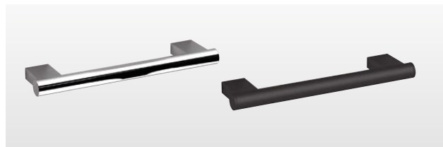
Lux Grab Bar 153237 Chrome £110 176083 Matt Black £160 W304 H24 D75mm - Bar Ø25mm
